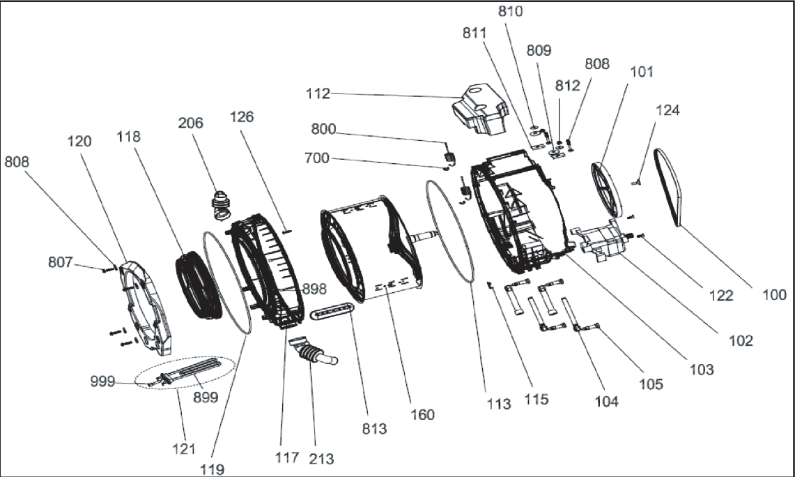
Exploded View 3 - Washing Group Parts
