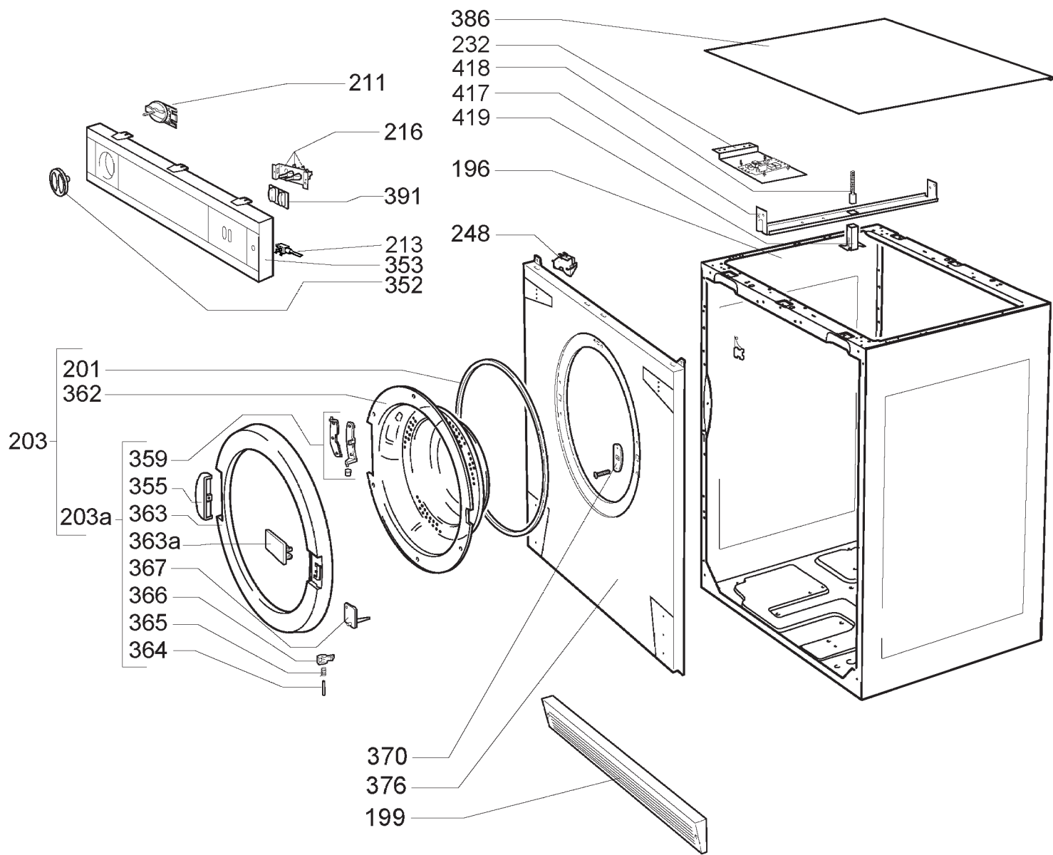
Exploded View 1
