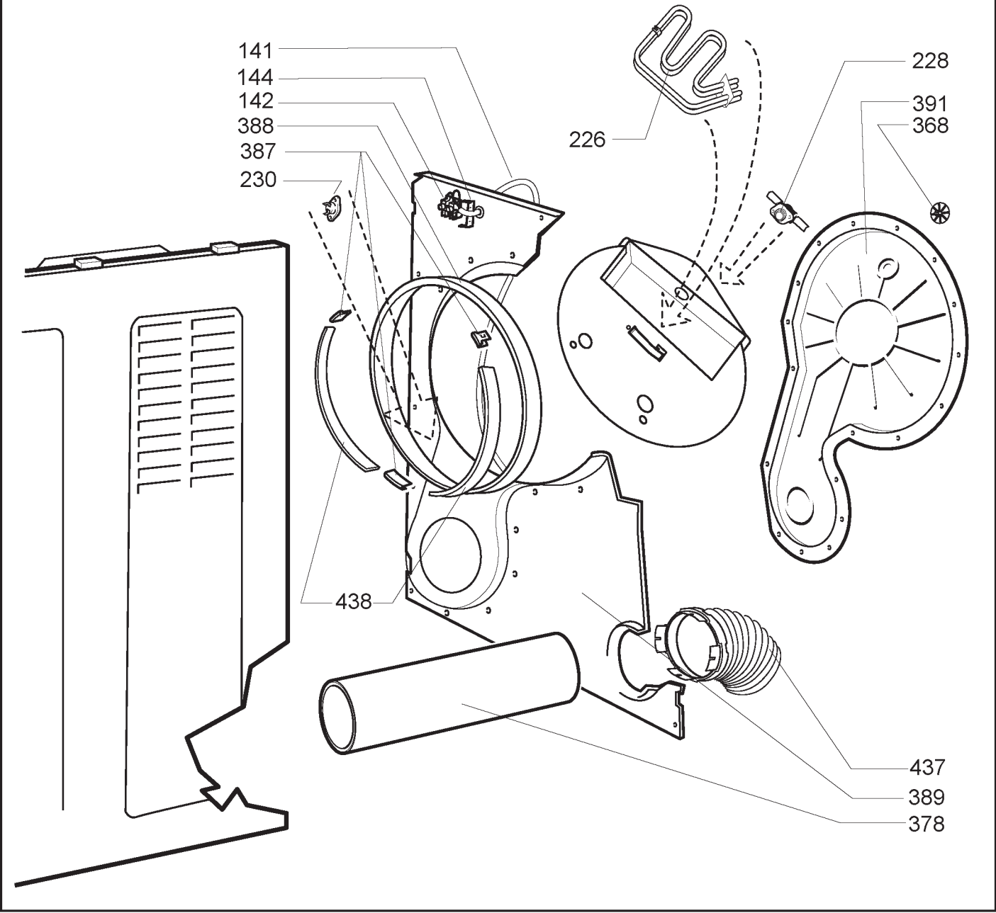
Exploded View 2
